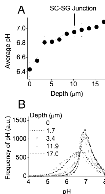
FIGURE 6 pH data of the stratum corneum. ( a ) Average pH as a function of depth. Each data point represents the average of the pH maps ( \leq 50 \times 50 \mu\text{m} ) taken from two different mouse skin samples. ( b ) Histograms of pH at different epidermal depths. The histogram data shows more clearly than a that two pH values are prevalent in the stratum corneum. With increasing depth, the frequency of acidic pH readings decreases. b indicates that the average pH in a increases with depth because of a decrease in the number of acidic regions contributing to the overall pH value.
