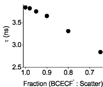
FIGURE 5 The effect of autofluorescence and/or scatter upon \tau of BCECF. Increasing background increases the detected modulation value. Background from our samples contributed <1% to the overall intensity measured.
